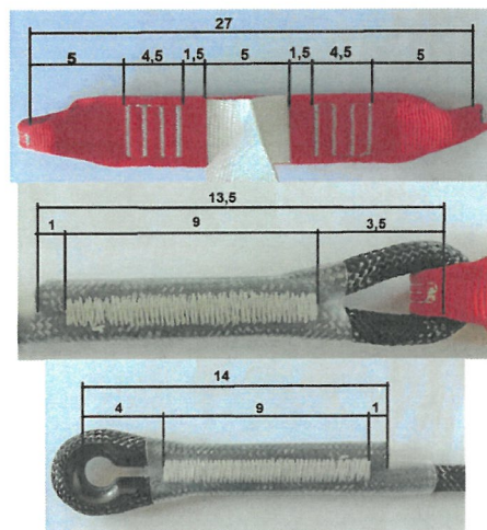
Dimensions in cm
